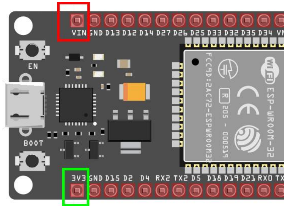
Abb. 1.6: ESP32-WROOM-32 – Versorgungsanschlüsse
